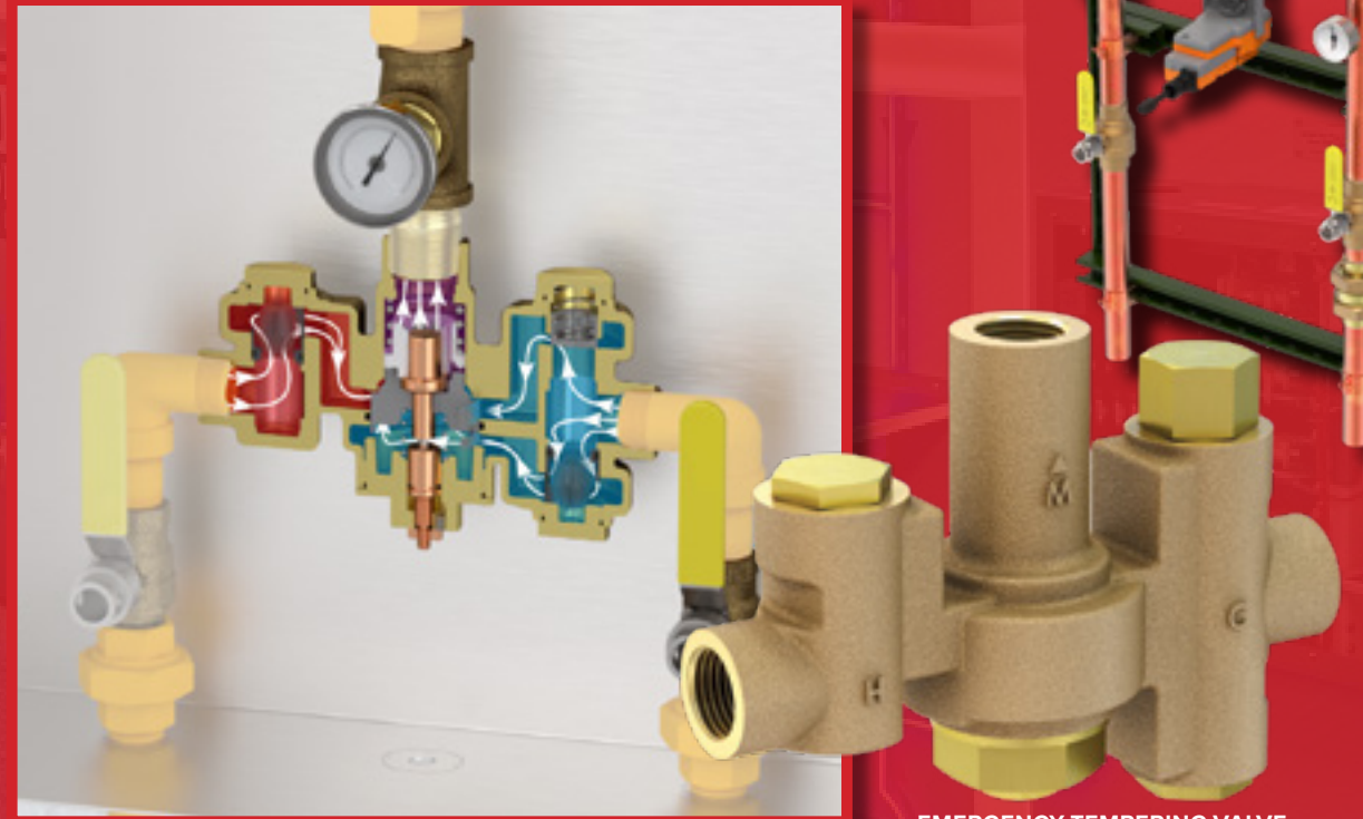
EMERGENCY TEMPERING VALVE Model No. ET71
