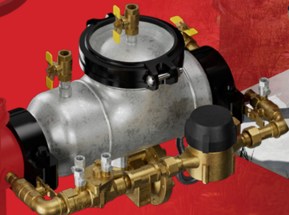
4" RPD BACKFLOW PREVENTER - OSY GXF Model No. 75RPD
